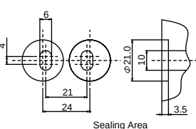
Sealing Area
